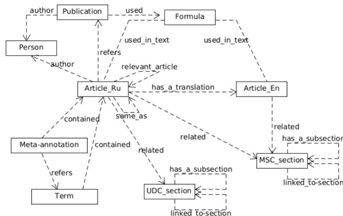
Figure 1: Diagram of LibMeta library data model.
