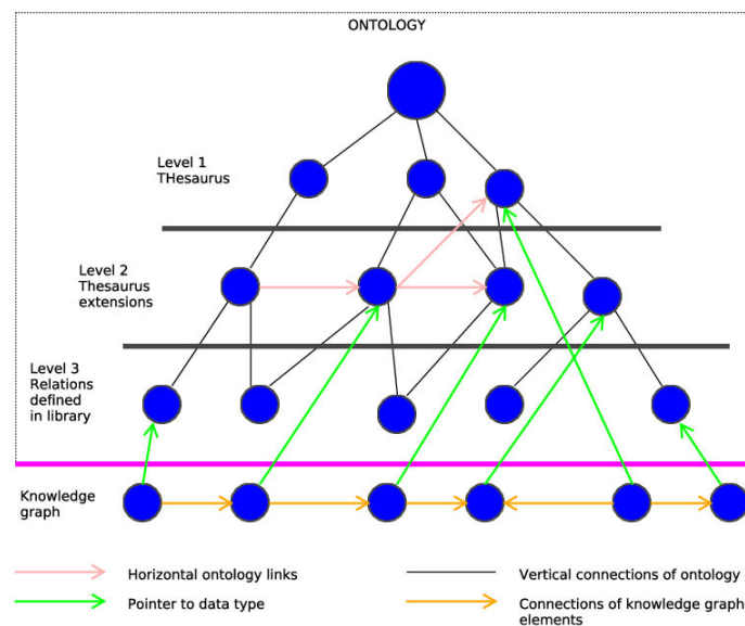
Figure 4: Scheme of three levels of the LibMeta library ontology.
